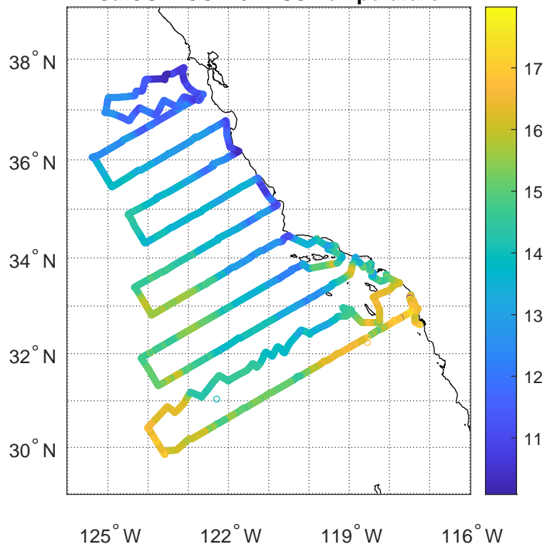
CalCOFI CC2204 - SS Temperature
