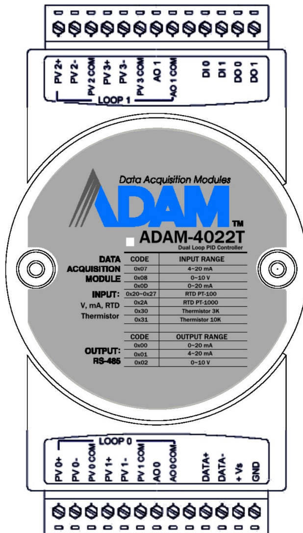
Fig. 1 ADAM-4022T Drawing
