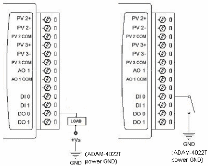
Fig. 3 Digital Input/Output Wiring Diagram
