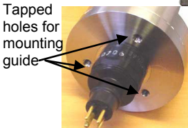
Remove plugs (2)
