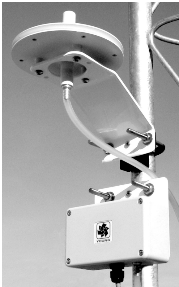
Barometer and Pressure Port
