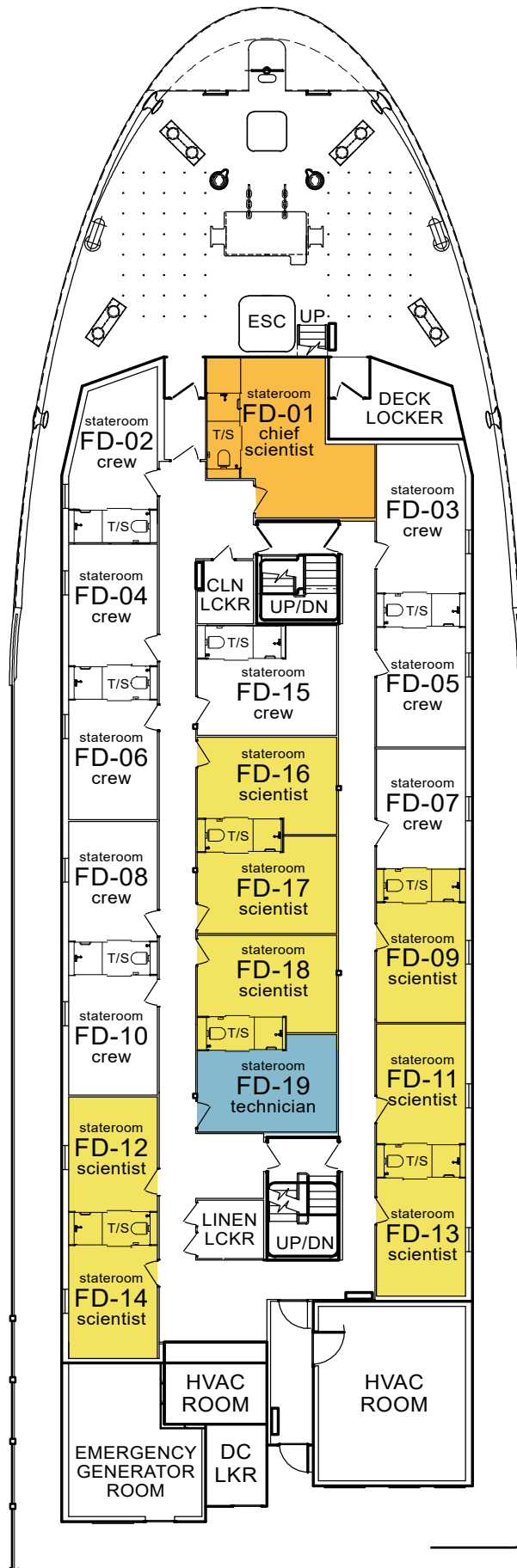
FOC'SLE DECK
